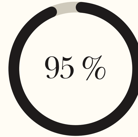
Analytical Thinking
